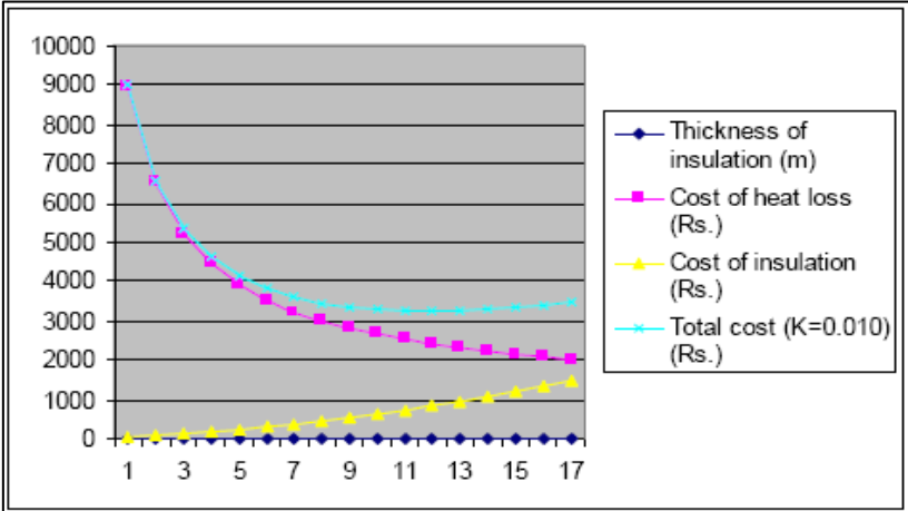
Fig 3: Variation of Cost with Thickness of Corrugated Asbestos Insulation
