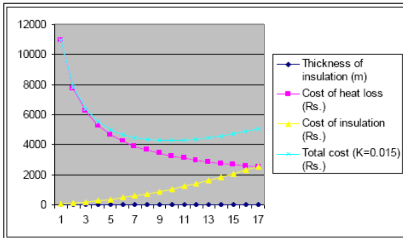
Fig 5: Variation of Cost with Thickness of Cellular Plastic Insulation (K=0.031)
