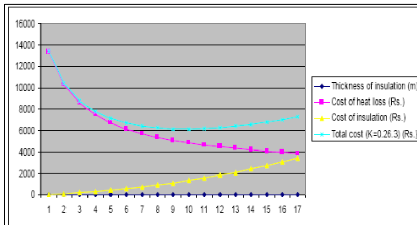
Fig 6 Variation of Cost with Thickness of Styrofoam Insulation (K=0.263)
