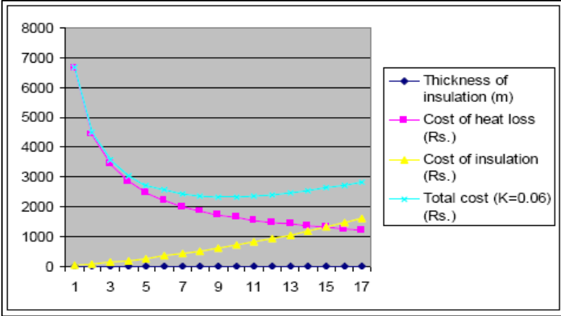
Fig 2: Variation of Cost with Thickness of Pearlite Insulation
